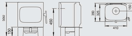
Jøtul F 105 with short legs
